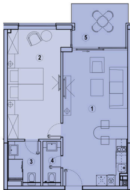
Apartment Type 4 One bedroom Apartment Total Sqm 56,5
